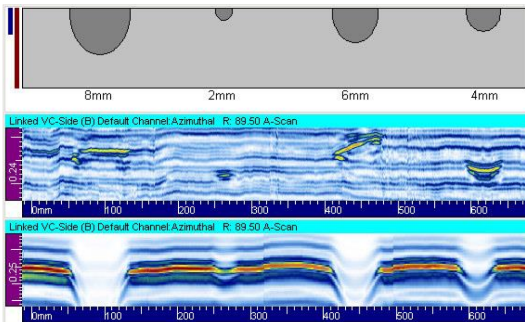
CIRCUMFERENTIAL SCANS ON A PIPE WITH SLOTS USING CREEPING WAVE AND ToFD
