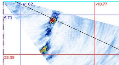
CORRESPONDING PAUT SPECULAR RESPONSES
