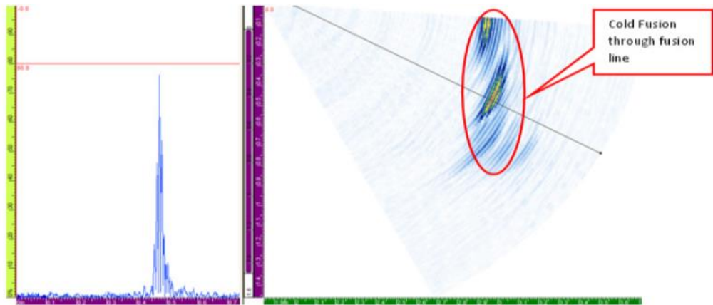
PA SCAN INDICATING COLD FUSION IN BF JOINT
