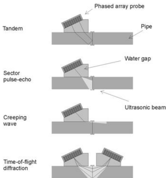
(Images from F. Hagglund, M. Spicer, M. Troughton "Development of Inspection Techniques for an Automated NDE Approach for Testing Welded Joints in Plastic PE Pipes.")
