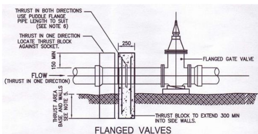
TYPICAL VALUE RESTRAINT RECOMMENDED IN WSAA CODE
