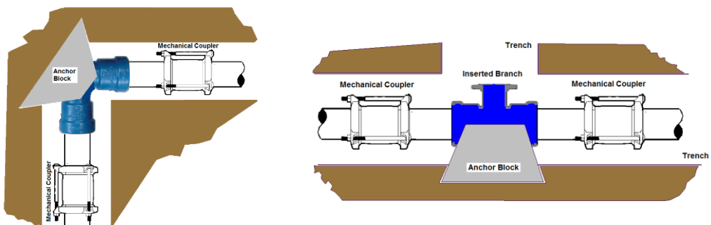
TYPICAL BEND INSERTION INTO AN TYPICAL BRANCH INSERTION INTO AN EXISTING PIPELINE
