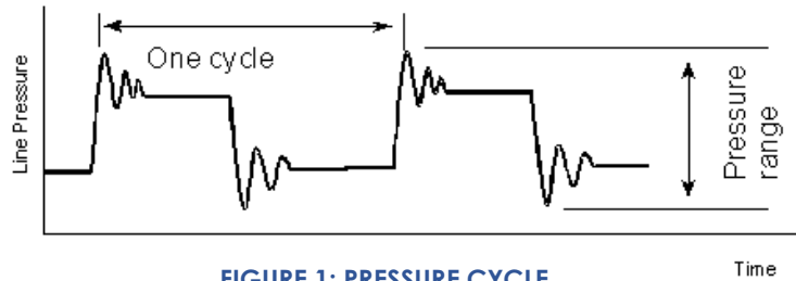
FIGURE 1: PRESSURE CYCLE
