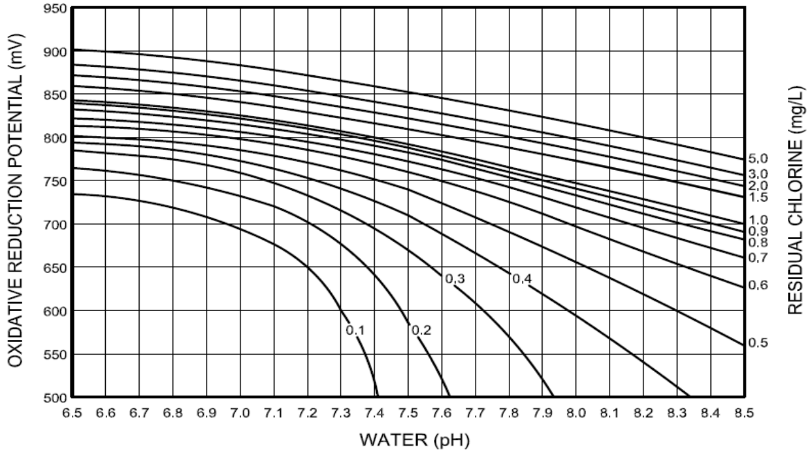
Chlorine and pH Water Quality Relationship
